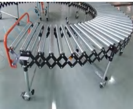
50*1.5mm galvanized steel roller
